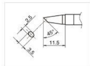
T39-BCF2535 Shape-BC hor:2.5mm vrt:3.5mm
