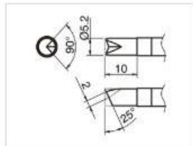
T39-BCR52 Shape-5.2BC with V-groove
