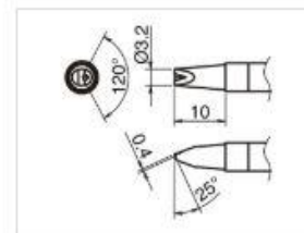
T39-DR32 Shape-3.2D with V-groove
