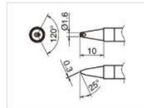
T39-DR16 Shape-1.6D with V-groove
