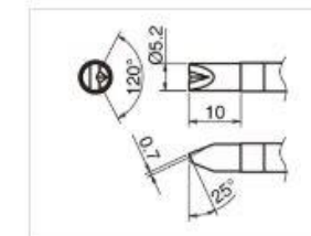
T39-DR52 Shape-5.2D with V-groove
