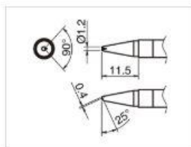
T39-BCR12 Shape-1.2BC with V-groove
