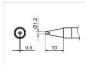
T39-D12 Shape-1.2D
