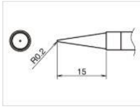
T39-BLL02 Shape-0.2BLL
