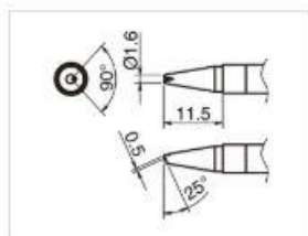
T39-BCR16 Shape-1.6BC with V-groove
