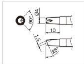
T39-BCR4 Shape-4BC with V-groove
