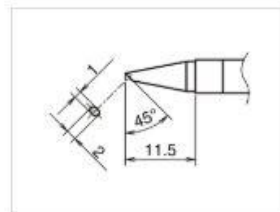
T39-BCF1020 Shape-BC hor:1mm vrt:2mm
