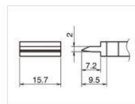
T39-SP157 Spatula 15.7mm
