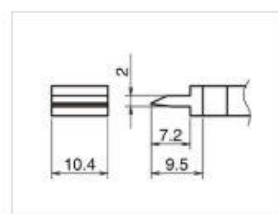
T39-SP104 Spatula 10.4mm
