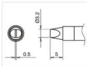
T39-DS32 Shape-3.2DS
