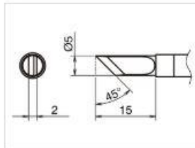
T39-K Shape-K
