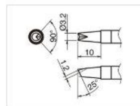
T39-BCR32 Shape-3.2BC with V-groove
