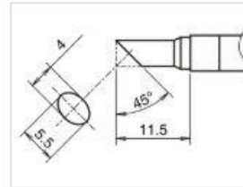
T39-C4055 Shape-C hor:4mm vrt:5.5mm
