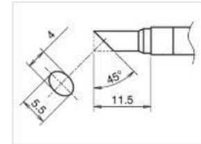
T39-CF4055 Shape-C hor:4mm vrt:5.5mm
