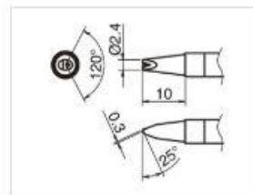
T39-DR24 Shape-2.4D with V-groove
