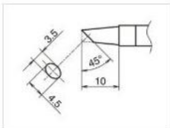
T39-BCF3545 Shape-BC hor:3.5mm vrt:4.5mm
