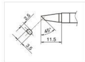
T39-BC2535 Shape-BC hor:2.5mm vrt:3.5mm
