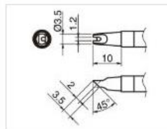
T39-BCR1235 Shape-BC with slot
